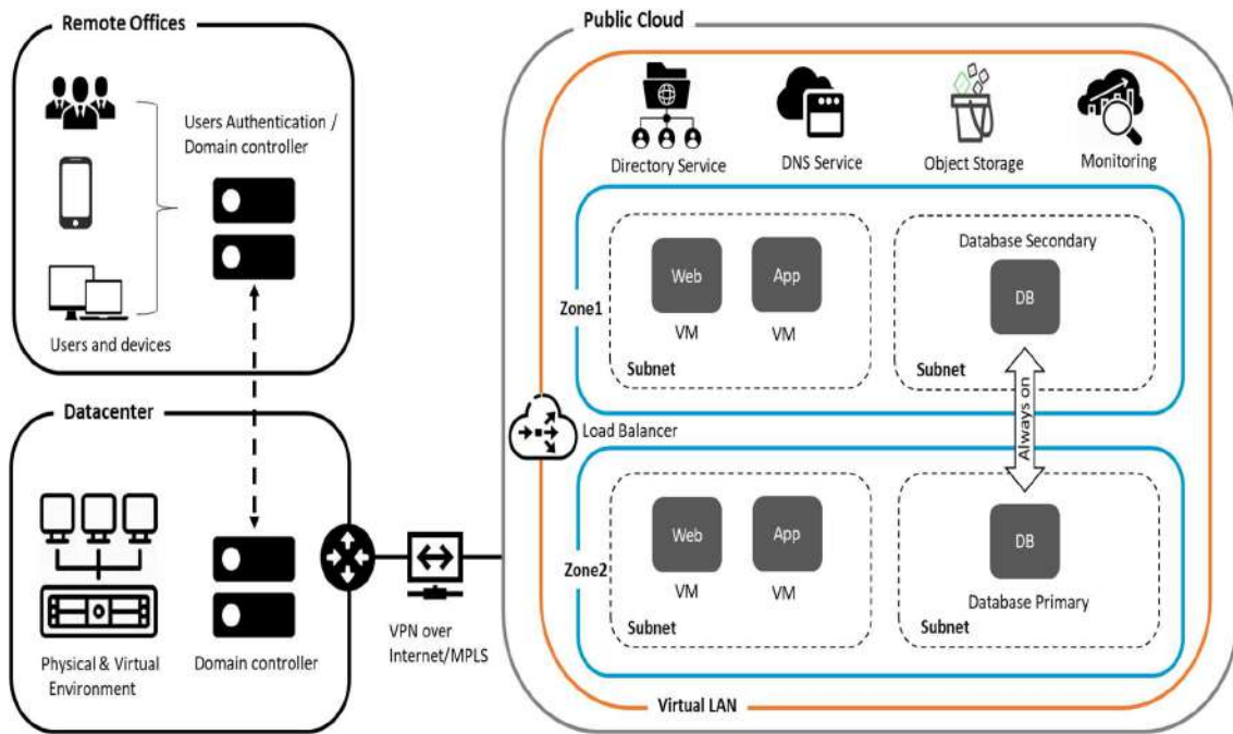
Figure 7: Database on Cloud
