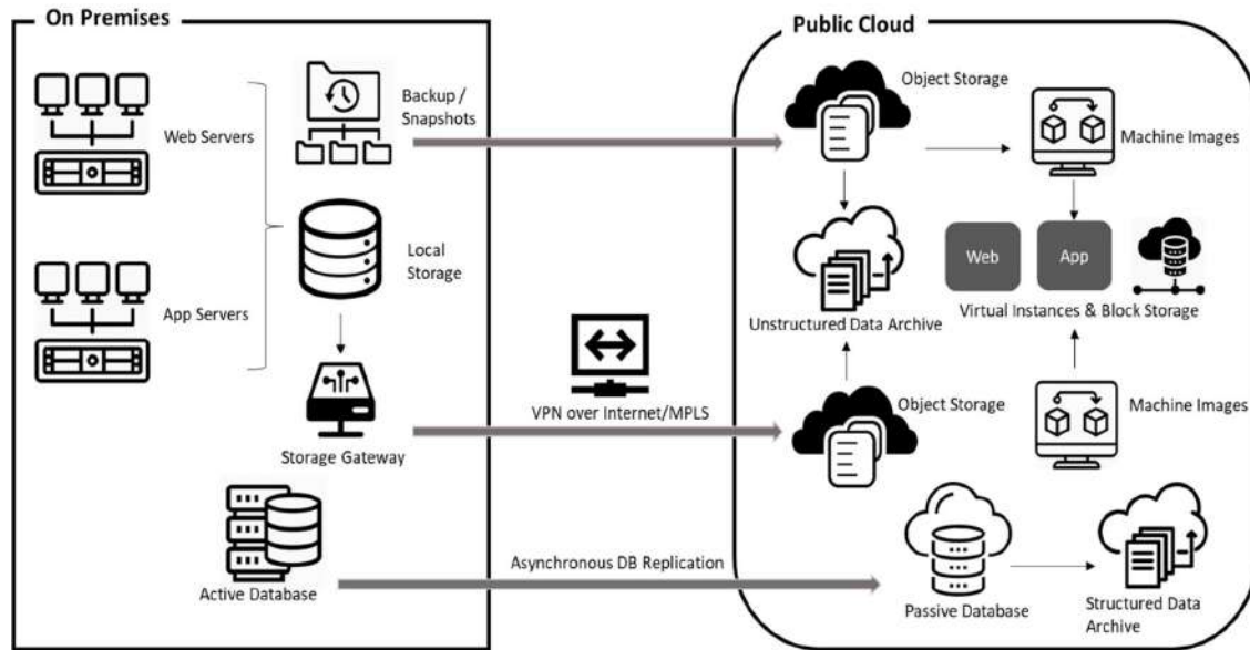
Figure 9: Backup & Archive/ Cold DR on Cloud with on-premise Primary DC
