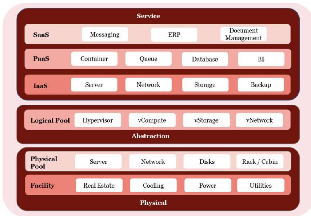
Figure 2: Service Orchestration
